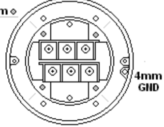
Terminal Block
