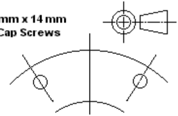
ZFK 8 Bolt Pattern
