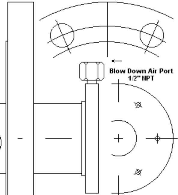
Bolt Pattern
