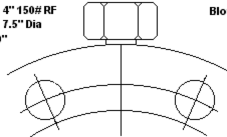
Bolt Pattern
